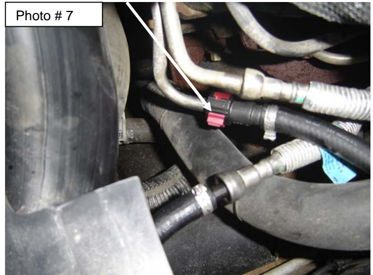
Plastic Disconnect Tool
