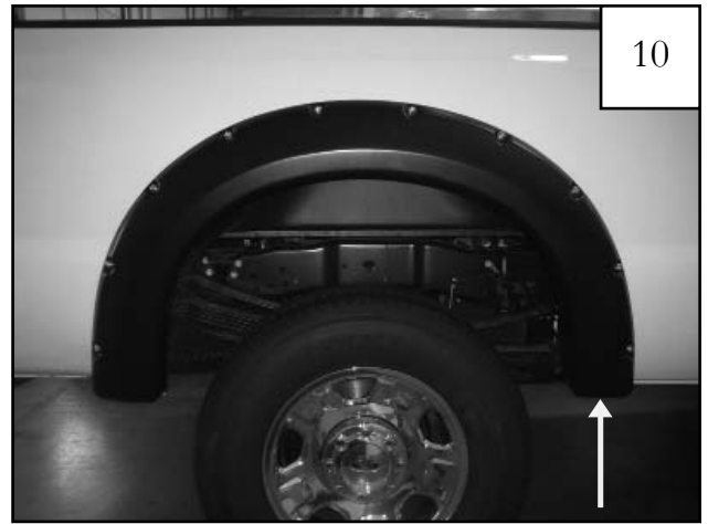
Place flare on fender and reinstall bolt removed in Step 5.
