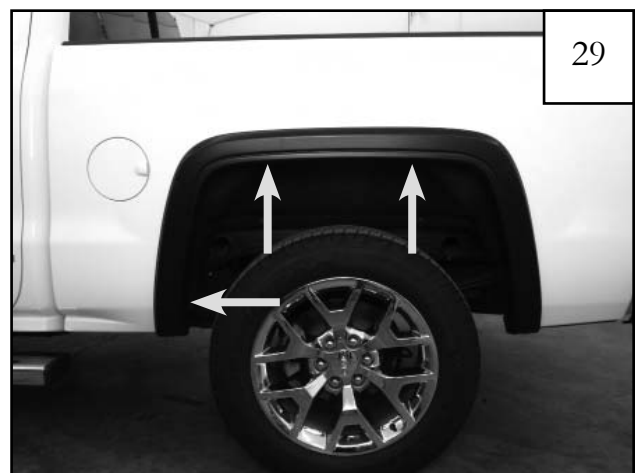
Hold rear flare up to wheel well to confirm fit. While holding flare on vehicle, install supplied screws (SW1-0068) into the 2 upper and 1 lower factory hole locations. Do not fully tighten at this time.
