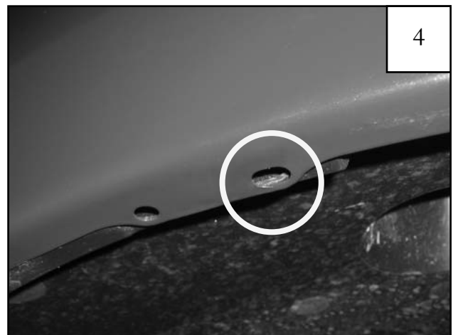
At location in step 3, there is a lip with two factory holes. One hole is a circle and one is an oval. The 1"x1.5" Black Tab and #10 U-Clip will be installed over the oval. The oval is the hole more toward the front of the vehicle.
