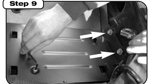
Once intake housing is set in position, re use two OE 13mm bolts on the side of the inner fender and use the two supplied button head on the base of the intake housing. Tighten with 5mm L-key.
