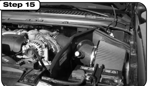
Place enclosed CARB EO sticker on a clean/smooth surface on or near the intake system. EO identification label is required in passing Smog Check inspection. Make sure all hoses and clamps are tight and that all electrical components are secure.
