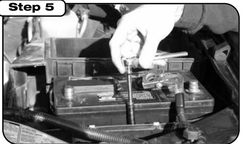
Remove battery hold down clamp from OE battery tray.
