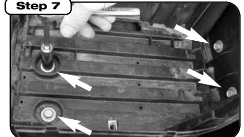
Remove four 13mm bolts as shown to take out OE air box.
