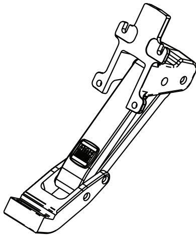
2 x2 10-02641-14 Idler linkage assembly
