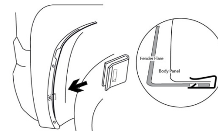
Push U-Clip
